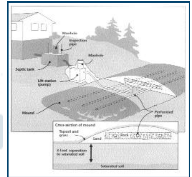
Figure 1. Cross section of a mound system. Illustration by James Kiehne.
